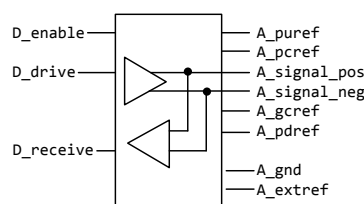
Figure 27 - Port Names for True Differential I/O Buffer
