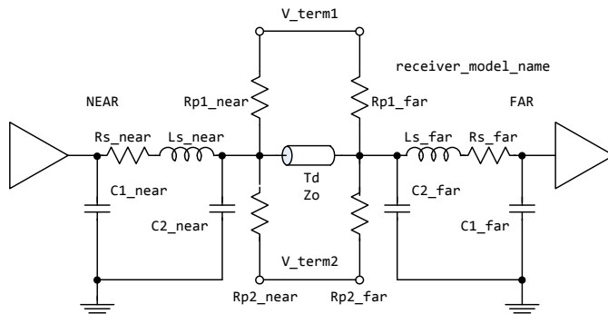
Figure 30 - [Test Load] Elements and Placement
