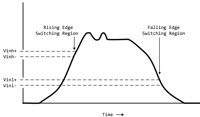
Figure 3 - Receiver Voltage with Hysteresis Thresholds
