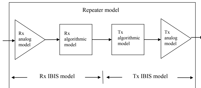
Figure 39 – Repeater model
