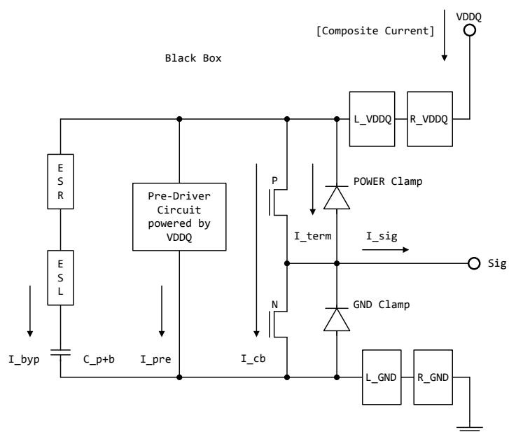
Figure 17 - [Composite Current] Internal Current Paths
