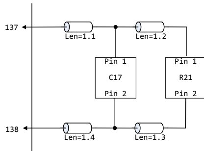
Figure 35 – Series Passive Components as Differential Termination
