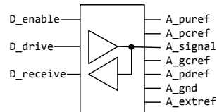
Figure 19 - Port Names for I/O Buffer
