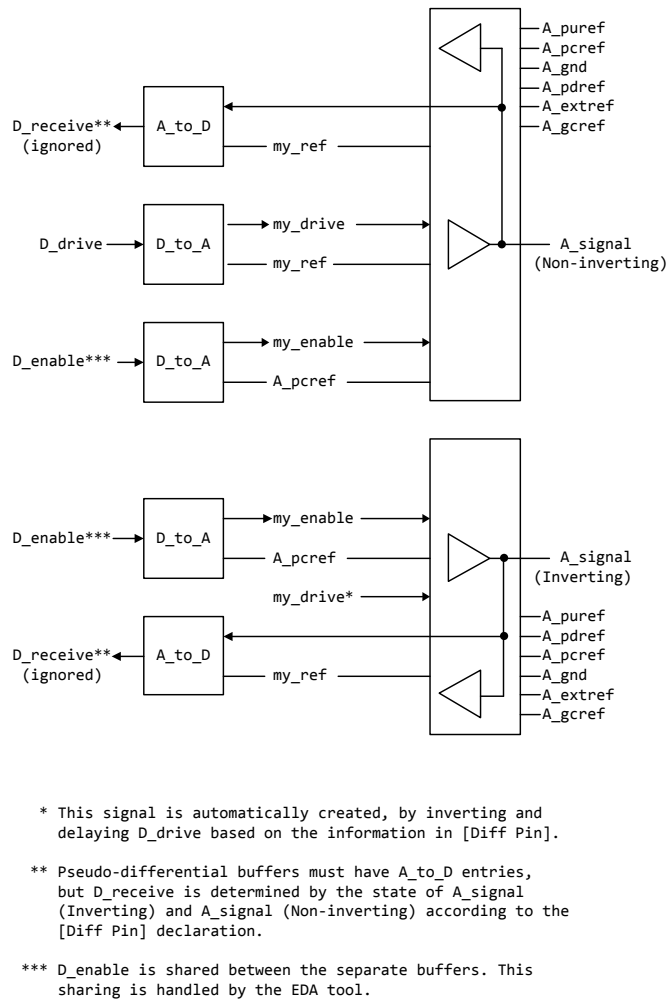
Figure 25 -Example SPICE, IBIS-ISS , Verilog-A(MS) or VHDL-A(MS) Implementation
