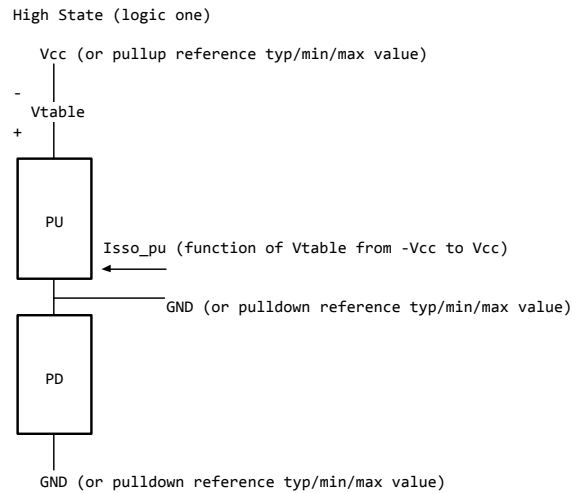
Figure 8 - High State (Logic One) Isso_pu Data Collection
